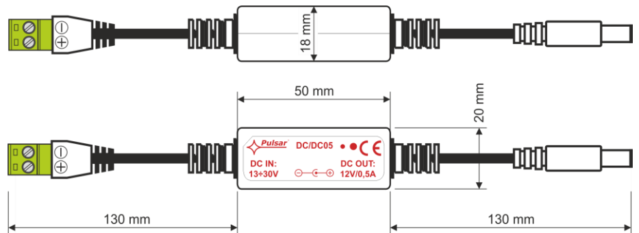
Fig.1. The mechanical diagram of the converter.
